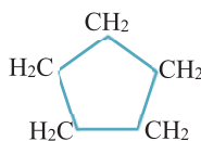
tsiklopentan \text{C}_5\text{H}_{10}
