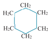
tsikloheksan \text{C}_6\text{H}_{12}
